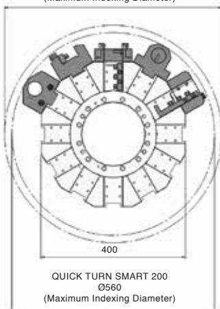
QUICK TURN SMART 250 Ø600 (Maximum Indexing Diameter)
